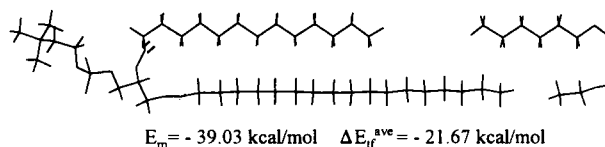
D. One C(18):C(14)PC complexed with one 1-octanol and one ethanol.
