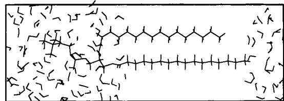
C. The hydration box for DPPC without ethanol :
