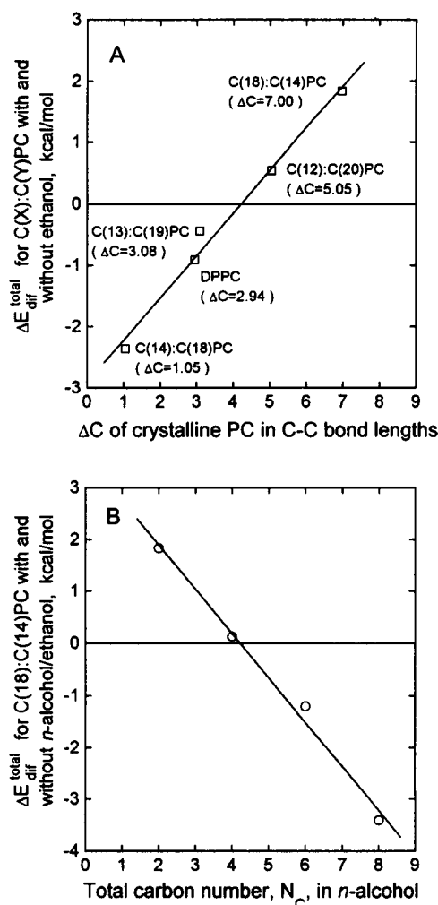
FIGURE 6 (A) The total stability energy difference of the mixed-chain PC bilayer is plotted against the \Delta C value. If the value of \Delta E_{\text{dif}}^{\text{total}} is negative for a given C(X):C(Y)PC specified by its \Delta C , this mixed-chain PC bilayer can be expected to undergo the partially interdigitated \rightarrow L_{\beta I} phase transition. (B) The total stabilization energy difference between the C(18):C(14)PC bilayer and the bilayer composed of a ternary complex of C(18):C(14)PC/ n -alcohol/ethanol is plotted against the total number of carbon atoms, N_c , in n -alcohol. The various n -alcohols are indicated in Fig. 4, and the total stabilization energy difference is defined in Table 1.
