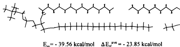
FIGURE 4 The simulated structures of C(18):C(14)PC complexed with (A) two ethanol, (B) one butanol and one ethanol, (C) one 1-hexanol and one ethanol, (D) one 1-octanol and one ethanol. The values of the steric energy and the overall averaged stabilization energy, \Delta E_{\text{st}}^{\text{ave}} = \frac{1}{2} (E_{\text{st}}^{\text{F-B}} + E_{\text{st}}^{\text{U-D}}) , are also given for each binary or ternary complex.
